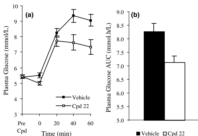
Figure 4. In vivo OGTT efficacy data for compound 22 (30 mg/kg po).
