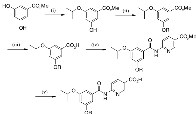
Scheme 1. General synthetic route to benzamides 13 and 16–25 . Reagents and conditions: (i) (CH 3 ) 2 CHBr, K 2 CO 3 , DMF (35%); (ii) Ph 3 P, DEAD, ROH, THF or RBr, K 2 CO 3 , DMF (60–80%); (iii) 1 M NaOH, THF/H 2 O (90%); (iv) (COCl) 2 , CH 2 Cl 2 , DMF (cat.) followed by methyl 6-aminonicotinate, THF, pyridine (70%); (v) 1 M NaOH, THF/H 2 O (90%).
